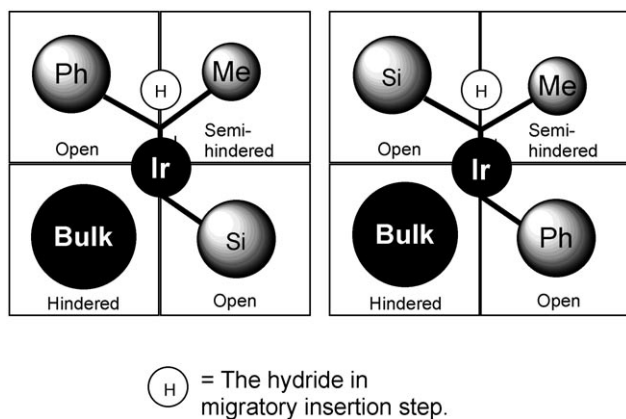
Figure 2. Schematic diagram of the selectivity model with substrates 5 (left) and 9 (right) coordinating onto the catalyst.
