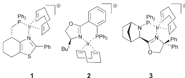
Figure 1. Ir complexes used in asymmetric hydrogenation of vinyl silanes. The anion in all cases is \text{B}[3,5-(\text{CF}_3)_2\text{C}_6\text{H}_3]_4^- ( \text{BAr}_\text{F} ).
